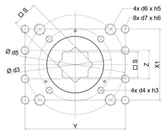
SAD/SAF 40-42
