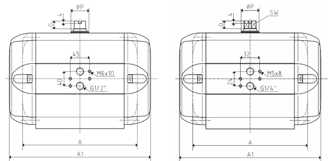
SAD/SAF 43-50
