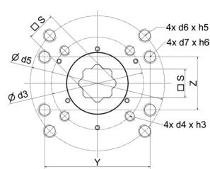
SAD/SAF 10-35
